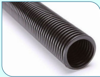
EVA VACUUM CLEANER HOSE Industrial vacuum cleaner & Swimming pool hose Temp. -50°C up to +60°C
