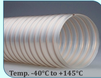
FLEXADUX HT PU POLYURETHANE HOSE FOR HIGH TEMPERATURE APPLICATIONS Wall Thick . 0.7/1/1.4 mm Temp. -40°C to +145°C (Short-term: +165°C)
