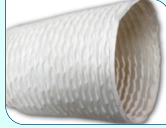
POLYESTER FABRIC HOSE PVC COATED - UV RESISTANT Heavy Duty Antistatic and Fire Retardant Range: 38 mm to 1000 mm Wall Thick.: 0.5 mm Temp. -20°C to 70°C
