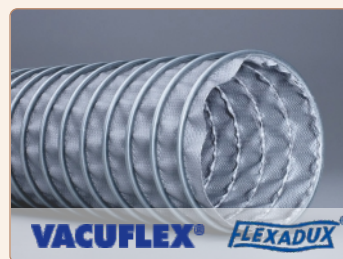
High Temperature Clip Silicon - German Wall Thickness: 0.4 mm Temp: -60°C to 300°C
